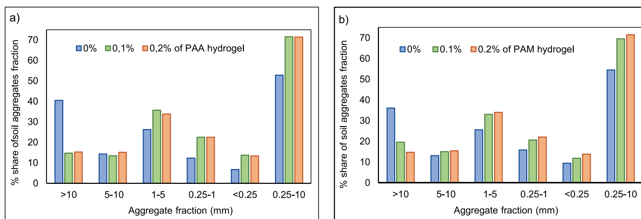
Fig. 3. The comparison of changes in the quantity of soil aggregates fractions after a) polyacrylate hydrogel (PAA), b) polyacrylamide hydrogel (PAM) application to loess soil; source: own elaboration based on literature data analysis PALUSZEK [2010] and PALUSZEK and ŻEMBROWSKI [2008]
