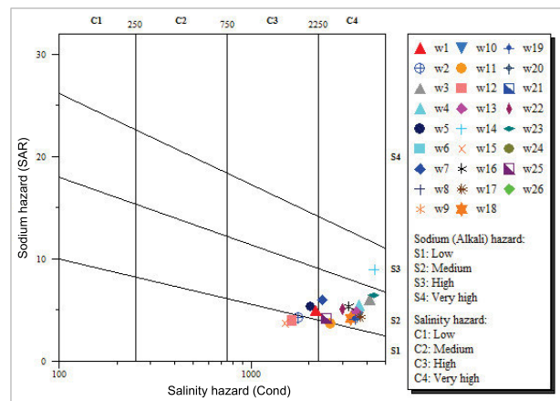
Fig. 3. Ghis-Nekor plain groundwater quality classification for irrigation, based on the Richards method; source: own study
