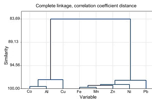
Fig. 3. The dendrogram of the distribution of heavy metals in sediment of the Bistrica River; source: own study
