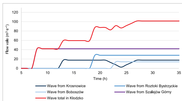
Fig. 13. Impact of reservoir outflow waves on the town of Kłodzko – pre-empted multifunctional reservoirs; source: own study
