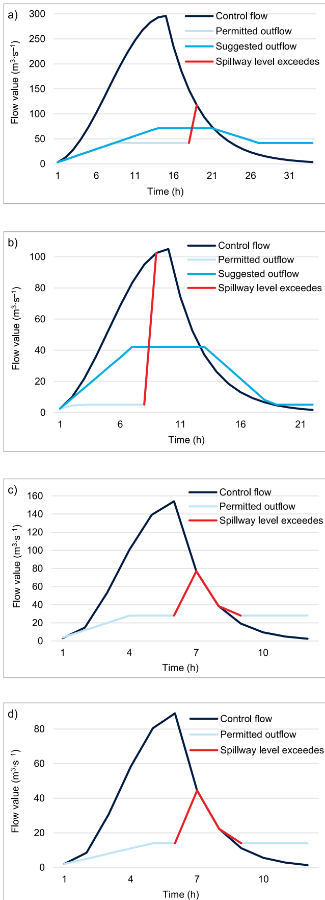
Fig. 6. Transformation of the control flow wave for the reservoirs: a) Sza-lejów Górny b) Krosnowice, c) Roztoki Bystrzyckie, d) Boboszków; source: own study
