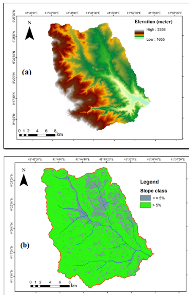
Fig. 3. Elevation (a) and slope class (b) map for suitable water harvesting site selection; source: own elaboration
