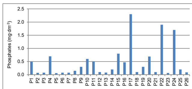
Fig. 13. Changes of phosphate concentrations in the studied well-water; P1–P26 = study wells as in Fig. 2 and Tab. 1; source: own study
