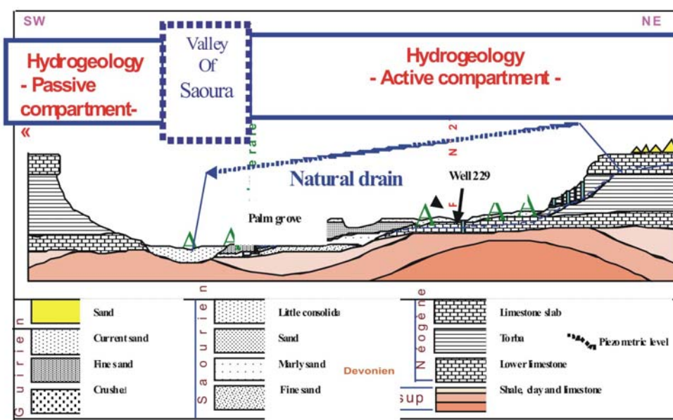
Fig. 4. Beni Abbes region hydrogeological section through Saoura; source: ROCHE [1973], modified by MERZOGUI et al. [2011]
