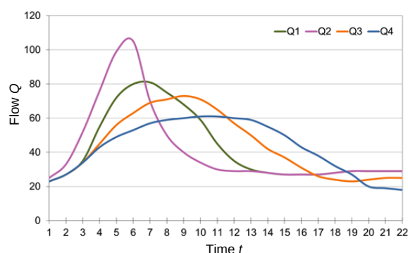
Fig. 2. Exemplary hydrograph of the food wave: Q1 – agricultural watershed, Q2 – municipal watershed, Q3 – forest watershed, Q4 – agricultural watershed with “small retention”; source: own study
