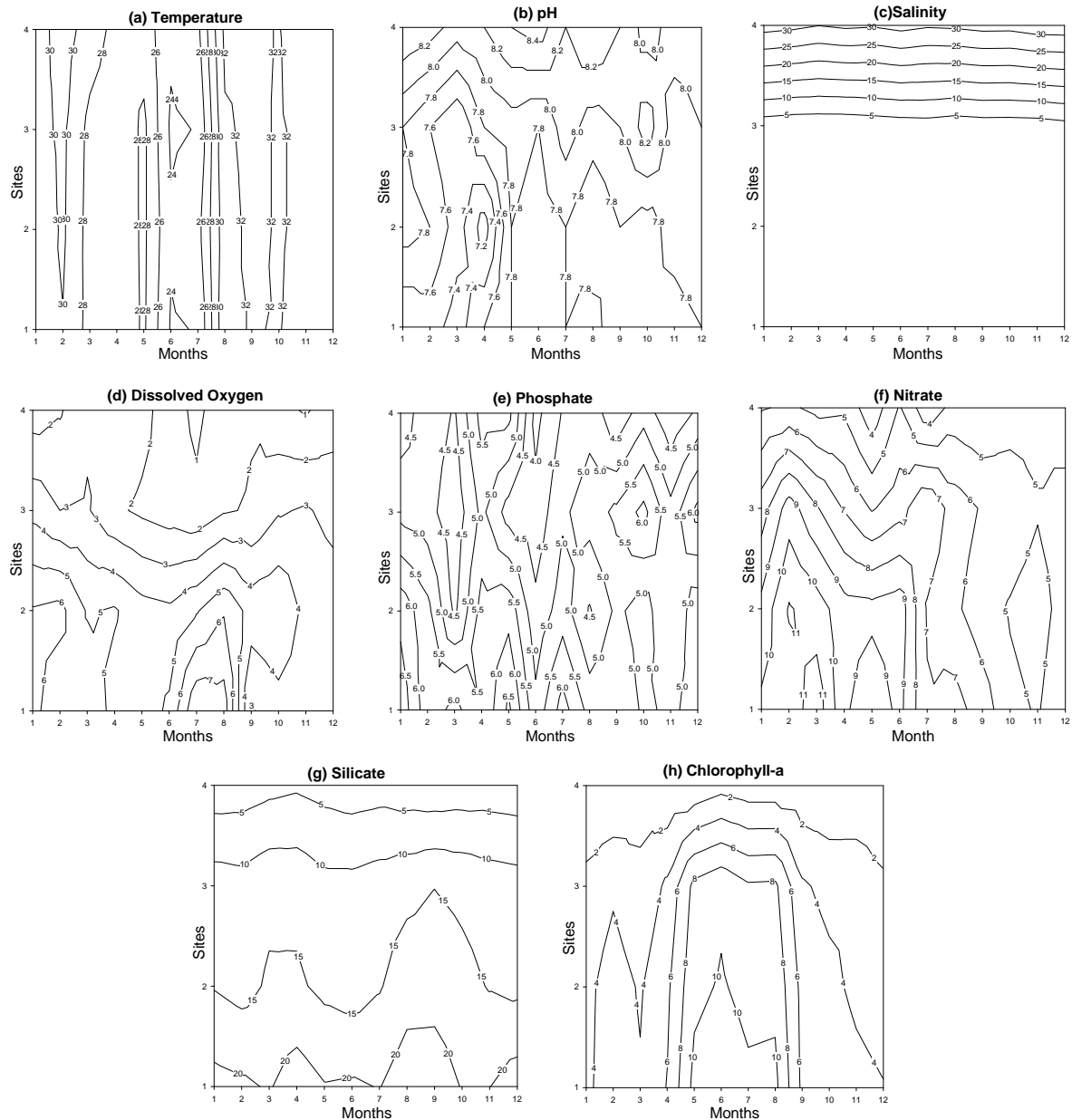
Fig. 4. Contours showing months wise variation in temperature, pH, salinity, dissolved oxygen, phosphate, nitrate, silicate and chlorophyll-a; sites: 1 – Zadeswar, 2 – Kukarwada, 3 – Bhadbuth, 4 – Ambata; months: 1 – July, 2 – August, 3 – September, 4 – October, 5 – November, 6 – December, 7 – January, 8 – February, 9 – March, 10 – April, 11 – May, 12 – June
